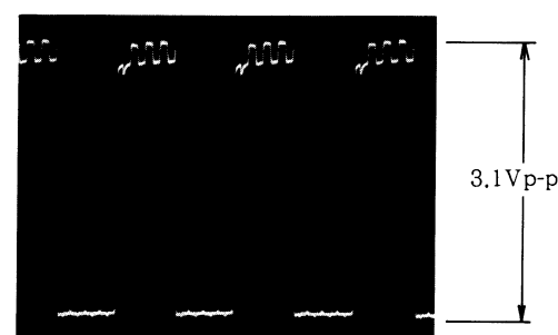
728 kHz bit clock (Pin ⑬ of IC01)
