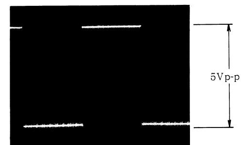
Word clock (Pin ⑨ of IC02)
