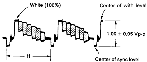
Fig. 7-10. Deviation adjustment
