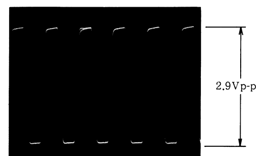
5.824 MHz master clock (Pin ⑫ of IC01)
