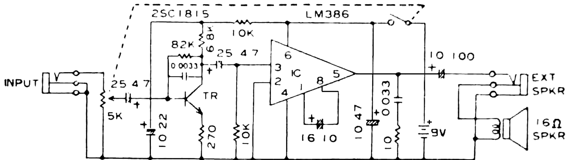
SCHEMATIC DIAGRAM OF MINI SPEAKER AMPLIFIER CAT. NO. 277-1008 B
