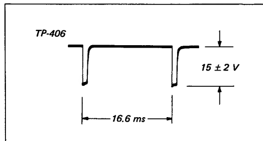
Fig. 6-6. Control track pulse check
