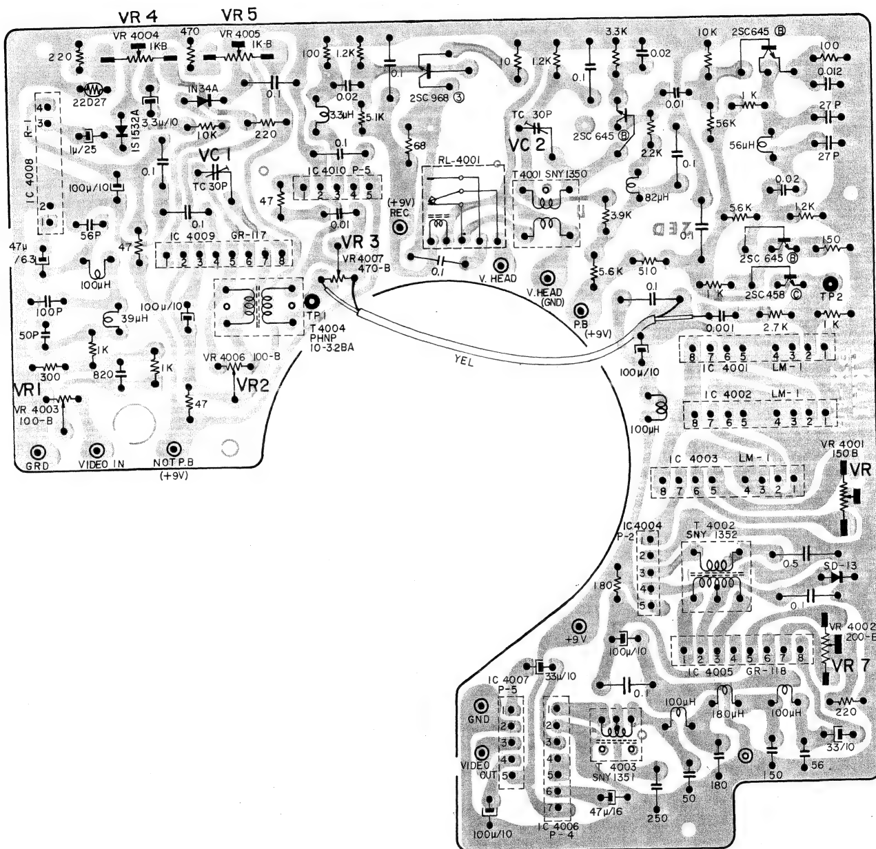
Fig. 1-48 Video Amplifier P.C. Board (PX-504)
