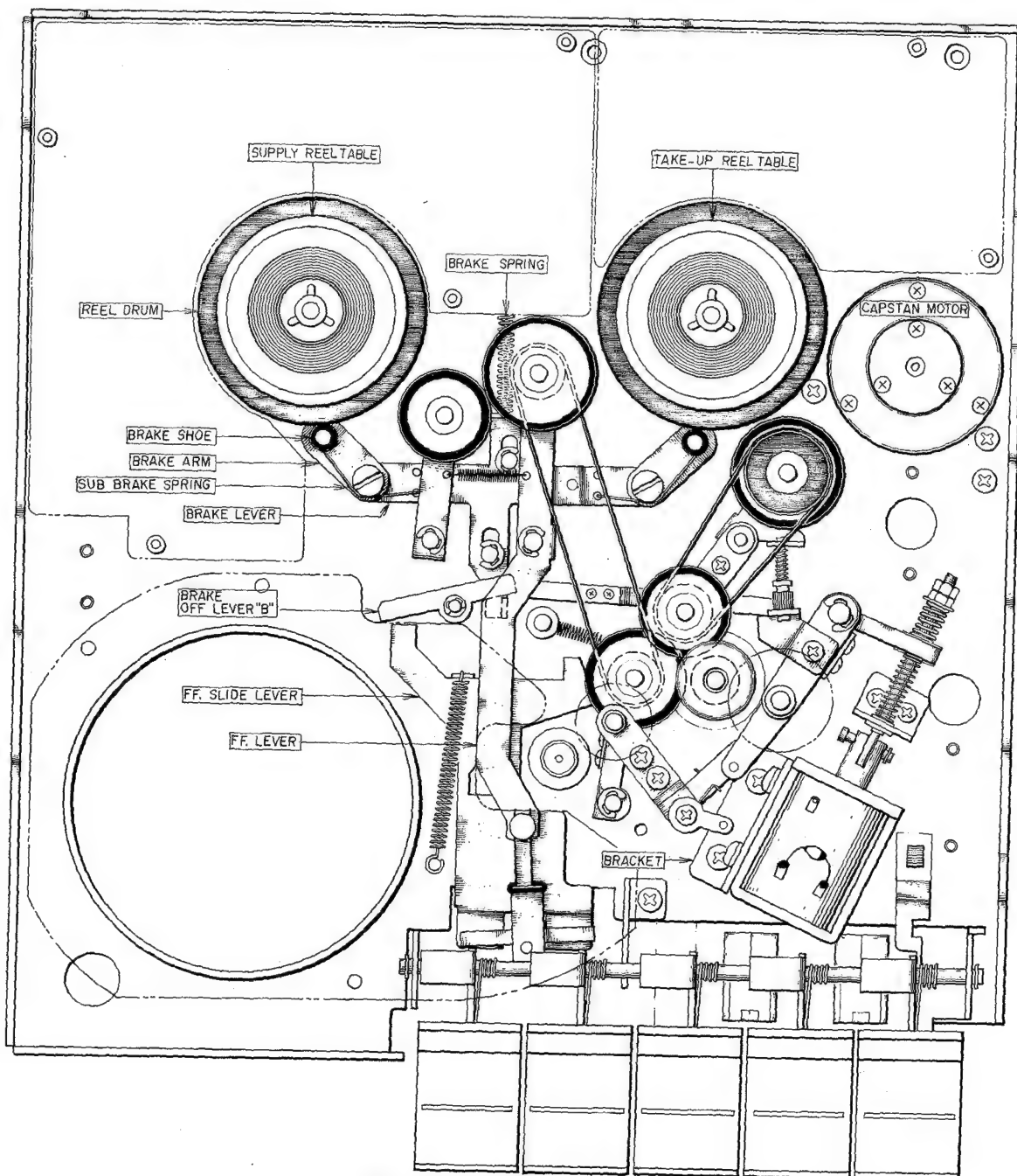
Fig. 1-28 Stop Mode
