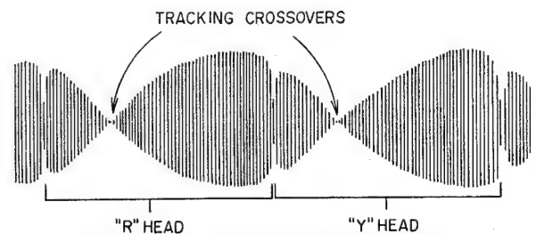
Fig. 1-23 RF Envelope with Guiding Error
