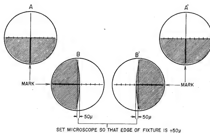
Fig. 1-11 Microscopic Views of Fixture
