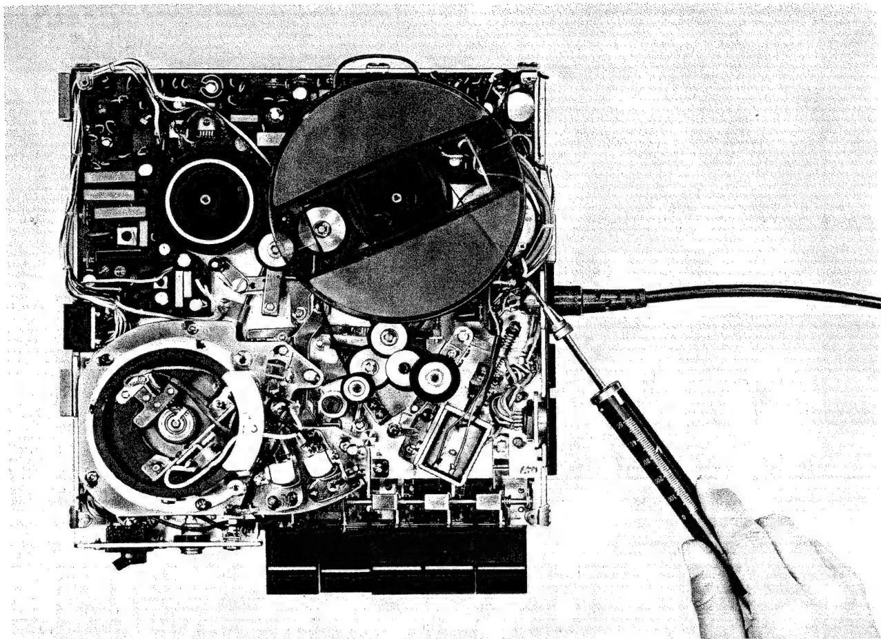
Fig. 1-31 Fast Forward Torque Measurement
