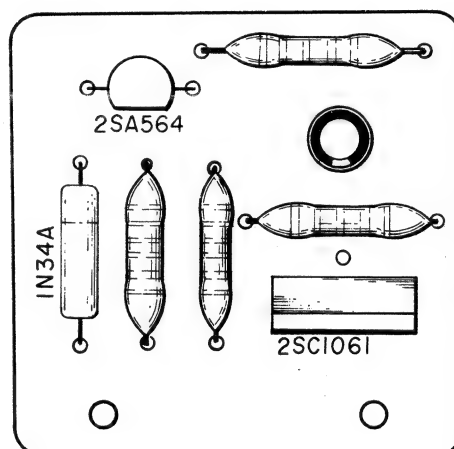
Fig. 1-54 Pinch Roller Solenoid Control P.C. Board (PX-508)
