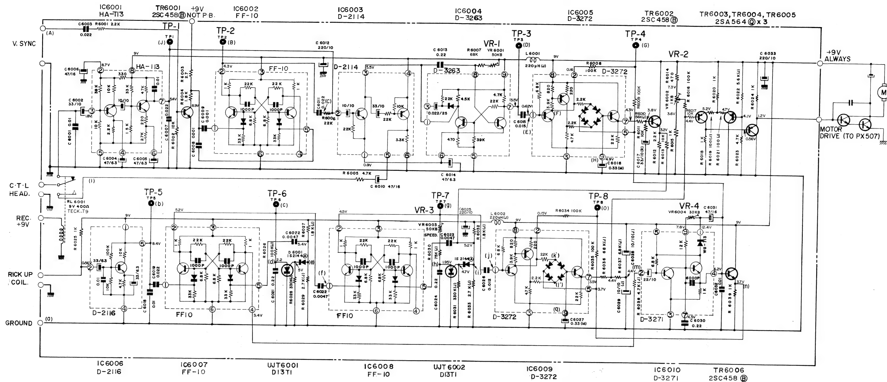
PXV (Recorder) SERVO P.C. BOARD PX-506 (PX-I-03)
