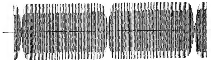
Fig. 1-27 RF Envelope with Incorrect Equalization
