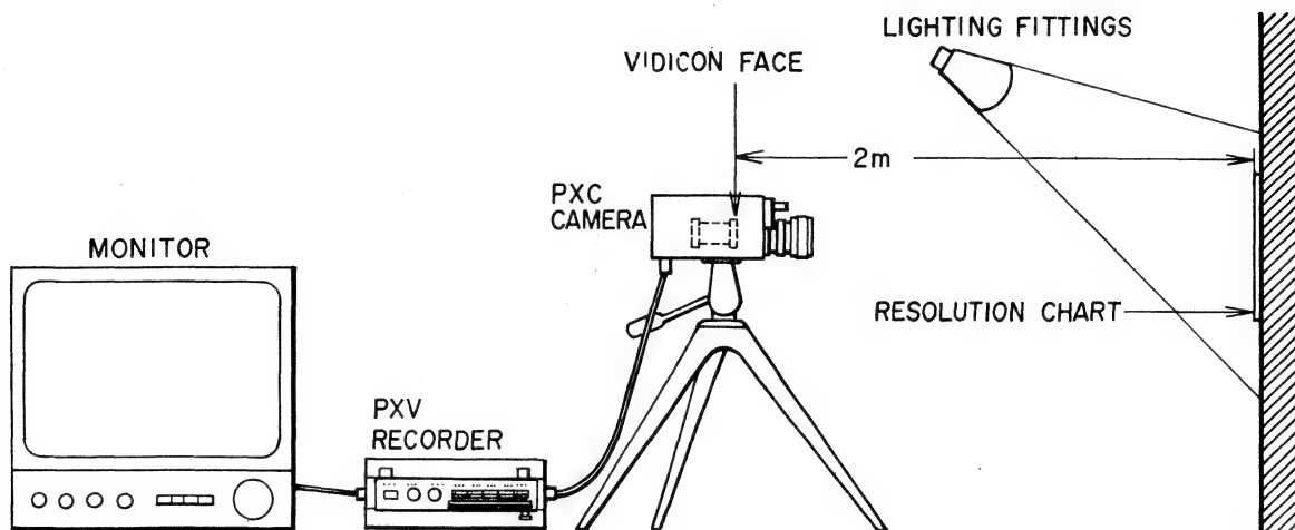
Fig. 2-1 Preparation for camera adjustment
