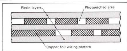
Cross-sectional diagram of FPC board
