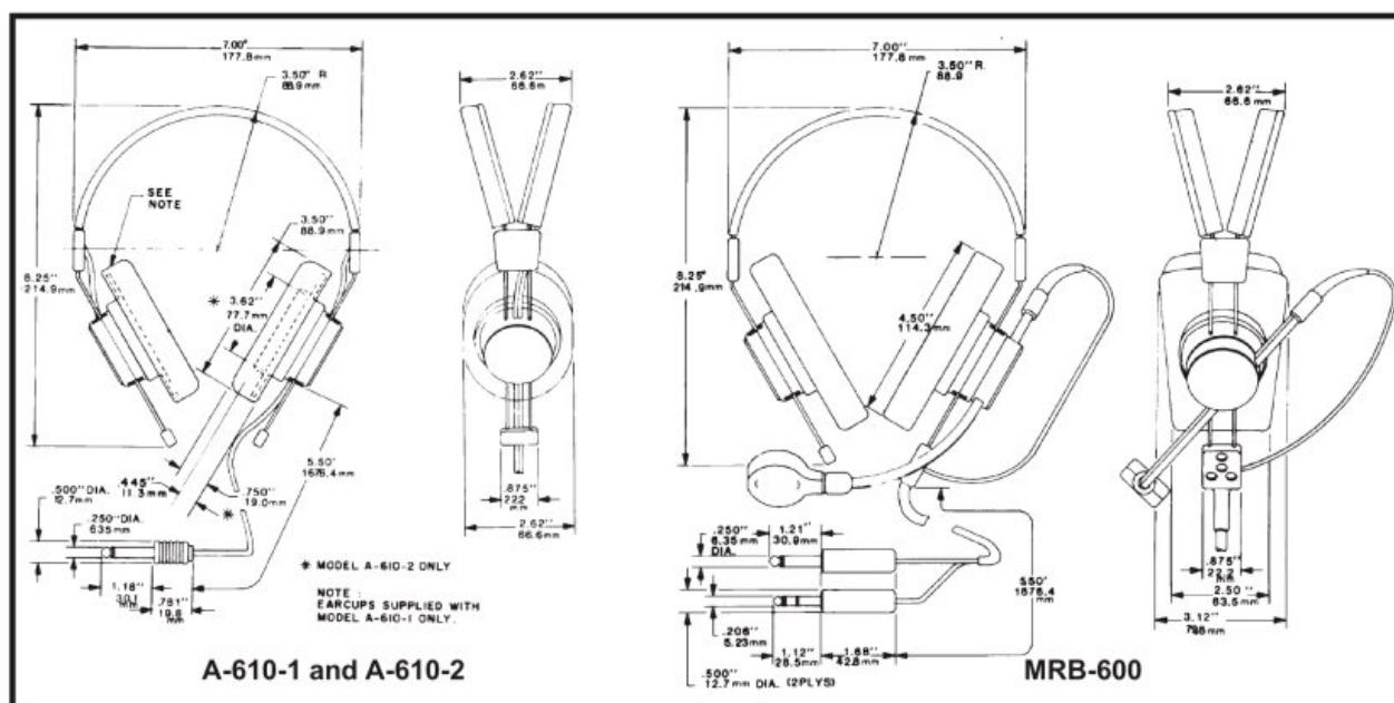
Dimension Drawings
