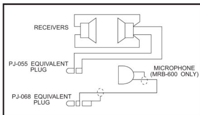
Schematic Diagram
