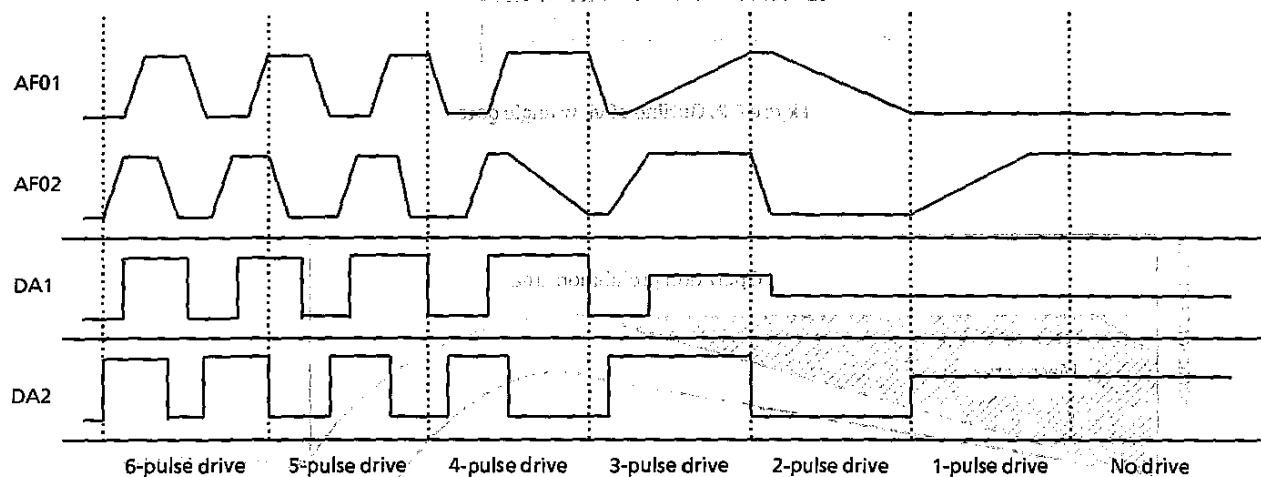
Figure 9-5. Driving pulses from microcomputer and motor driving pulses
