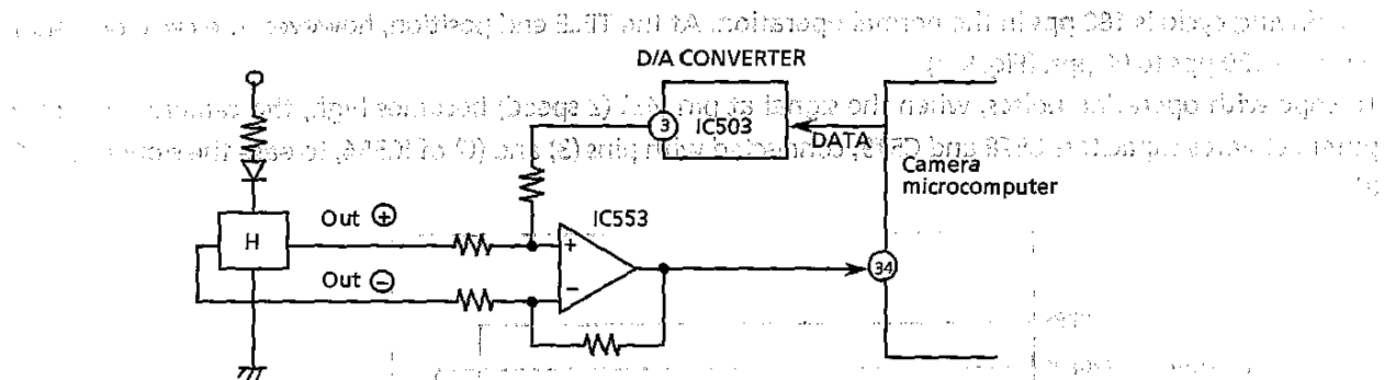
Figure 9-10. Hall sensor block diagram
