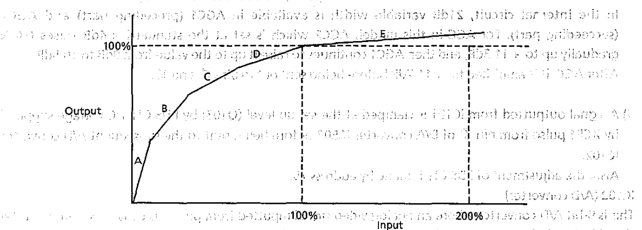
Figure 7-4. \gamma correction
