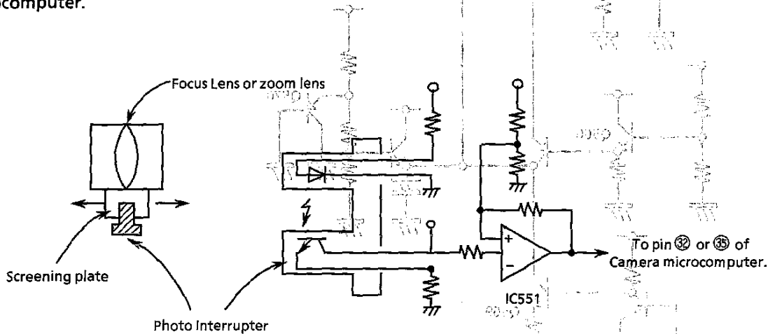
Figure 9-9. Photo interrupter block diagram
