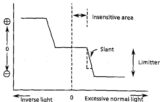
Figure 10-5. Limiter function
