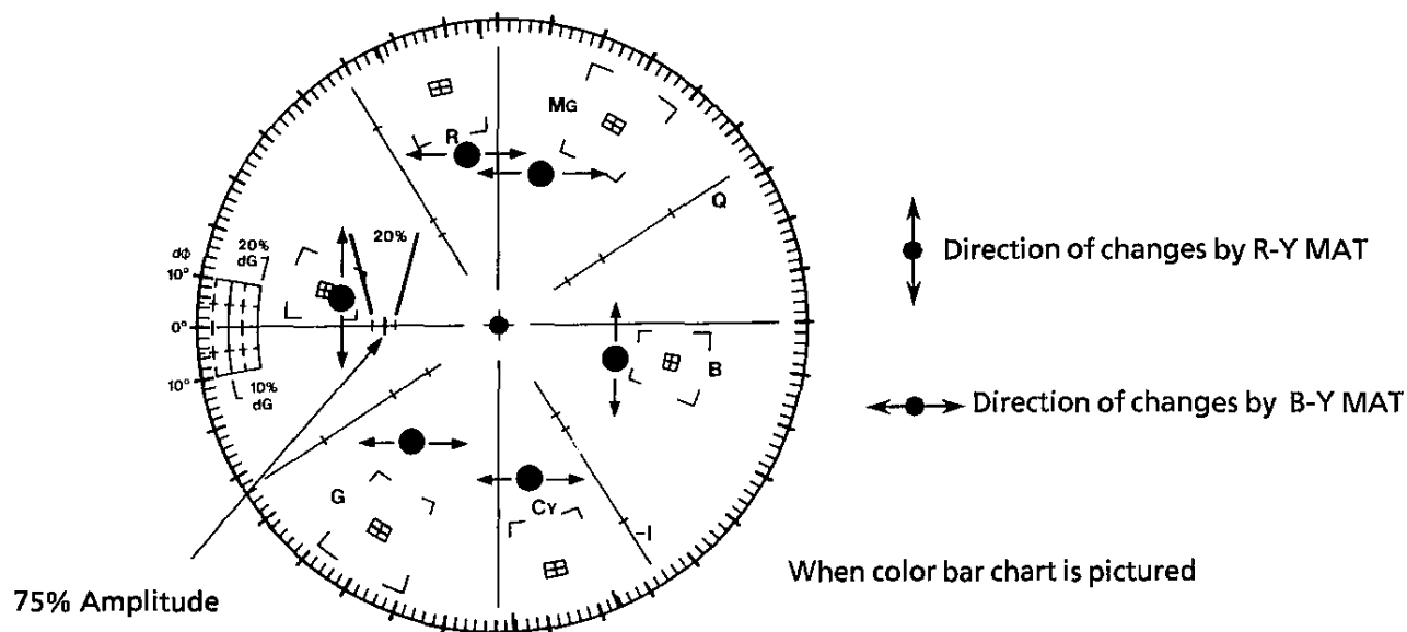
Figure 7-8. Hue Control
