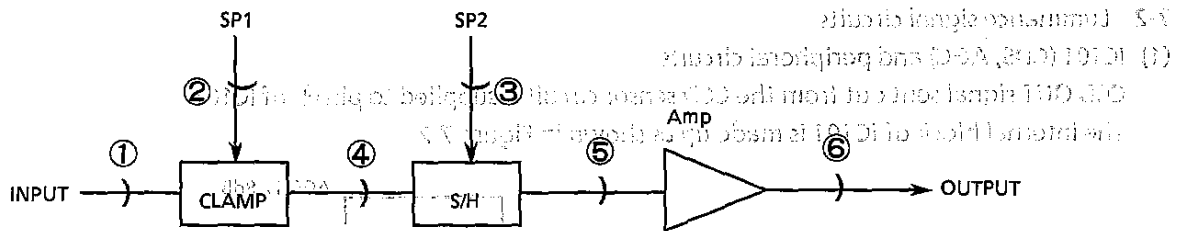
Figure 7-3(a). CDS circuit
