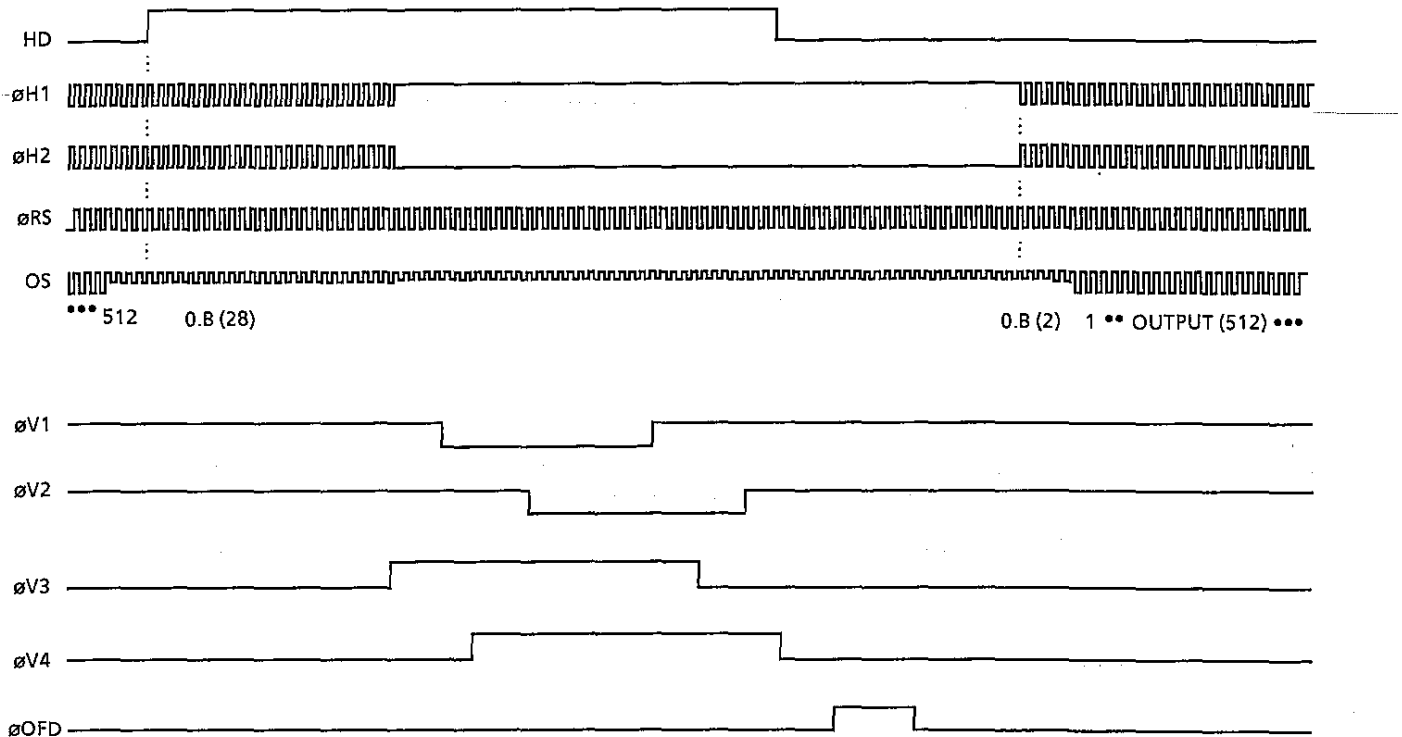
Figure 5-7. Horizontal Transfer Timing Chart
