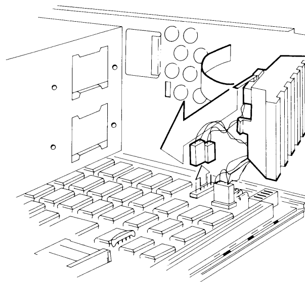
Figure 7-27. Removing the Speaker/Board Guide Assembly.
