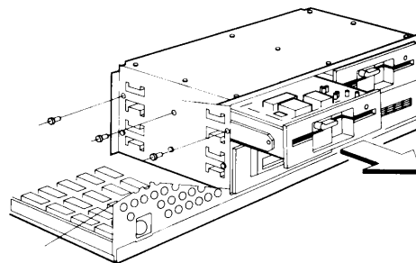
Figure 7-43. Removing Mass Storage Device A.
