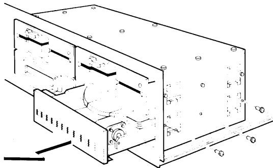
Figure 7-47. Removing Mass Storage Device C.
