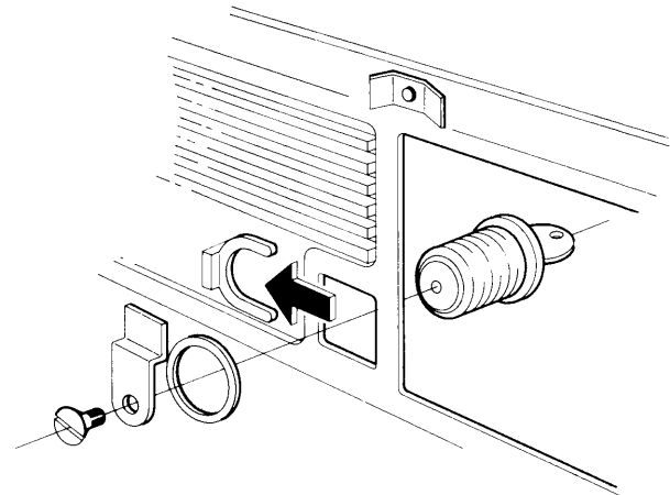
Figure 7-25. Removing the Security Lock.
