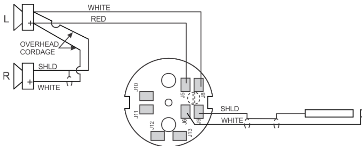
FIGURE 7. Airman 760 Headphone Model -200 Wiring Diagram
