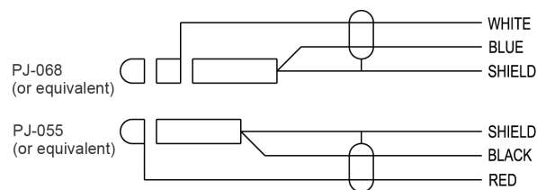
FIGURE 9. PJ068 and PJ055 Connector Wiring, 750 Model -200, -212, -300
