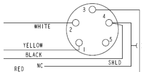
FIGURE 11. XLR Connector Wiring, 750 Model -205, -208, -210
