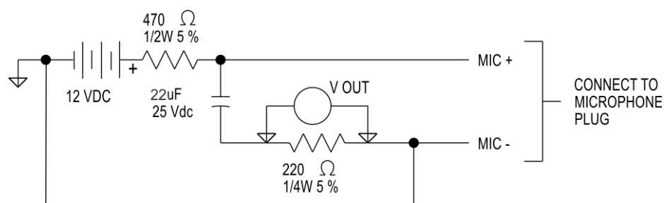
FIGURE 1. Airman 750 Headset Boom Microphone Sensitivity Check Test Circuit
