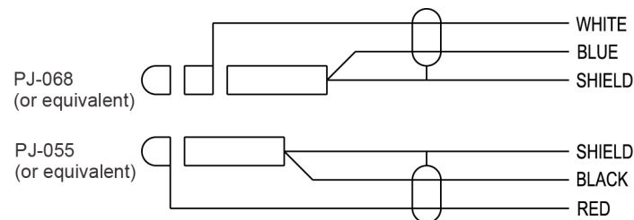
FIGURE 17. PJ055 and PJ068 Connector Wiring, 750 Model -220
