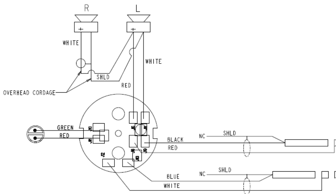
FIGURE 1. Airman 750 Headset Model -200, -220, -300 Wiring Diagram
