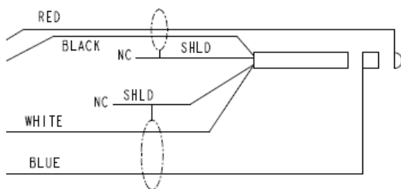
FIGURE 13. PJ-068 Connector Wiring, 750 Model -218
