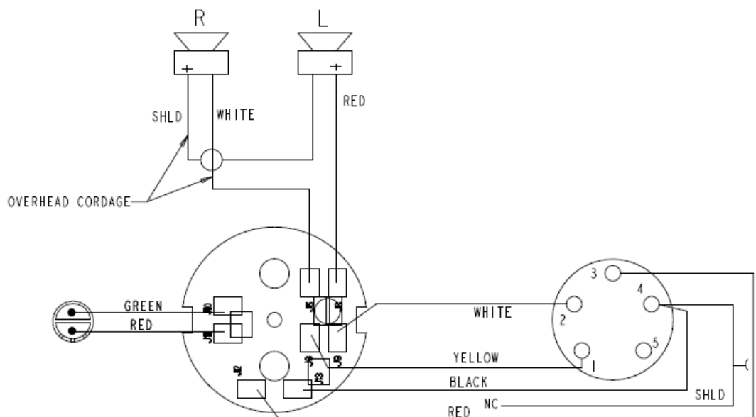
FIGURE 2. Airman 750 Headset Model -210 Wiring Diagram
