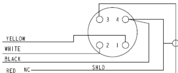
FIGURE 15. XLR Connector Wiring, 750 Model -219
