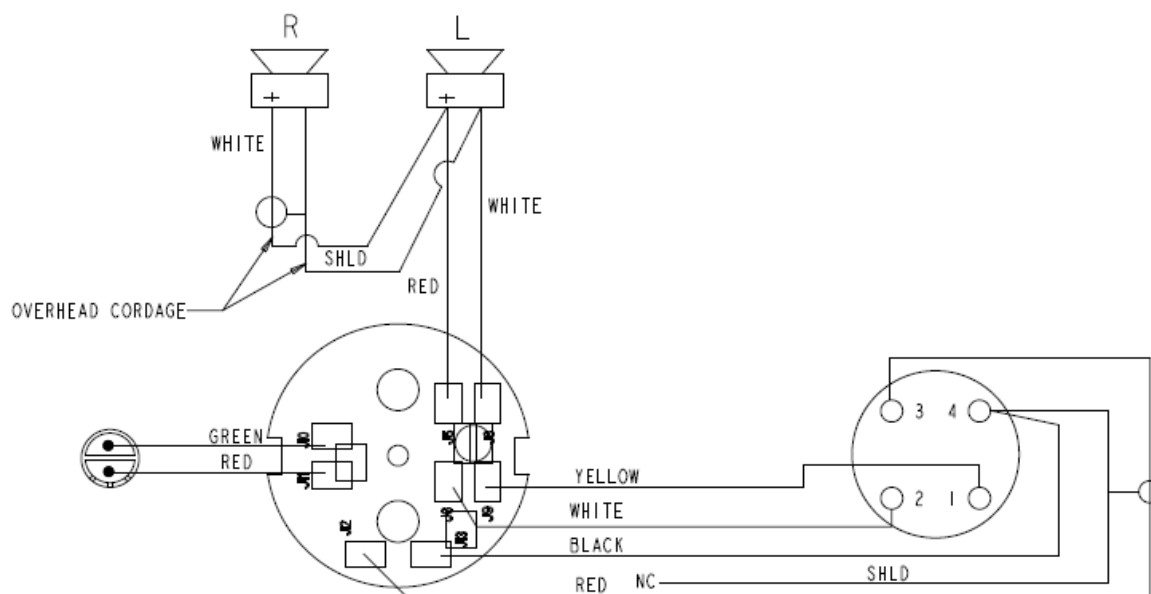
FIGURE 6. Airman 750 Headset Model 219 -Wiring Diagram
