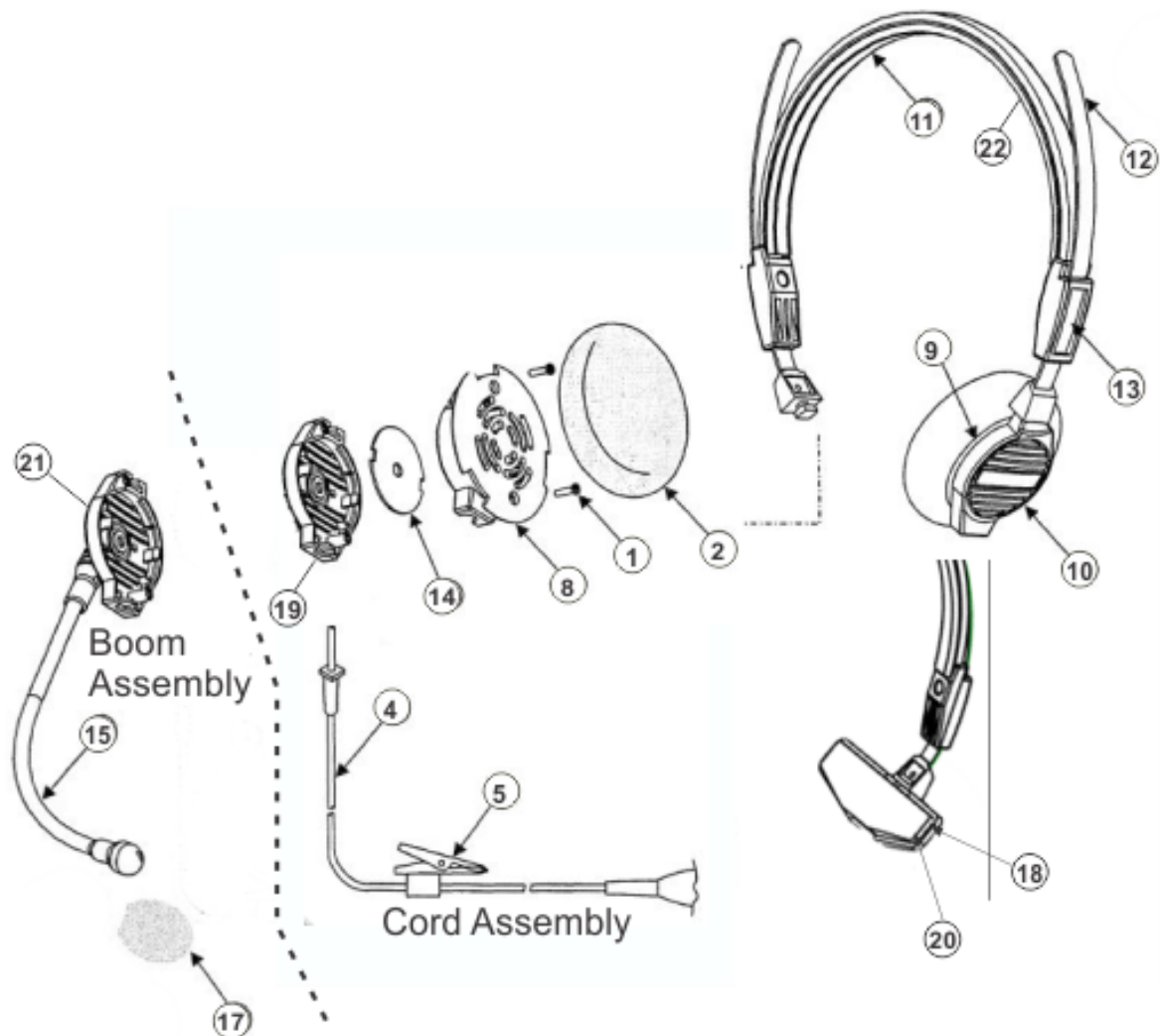
FIGURE 1. Airman 750/760 Series-200/300 Exploded View
