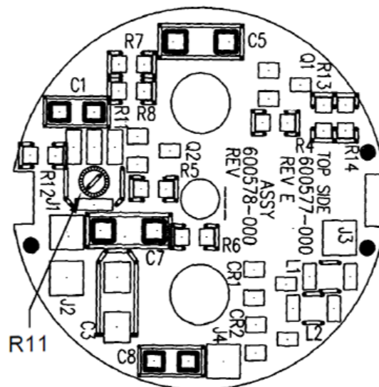
FIGURE 3. Gain Adjustment Potentiometer (R11)
