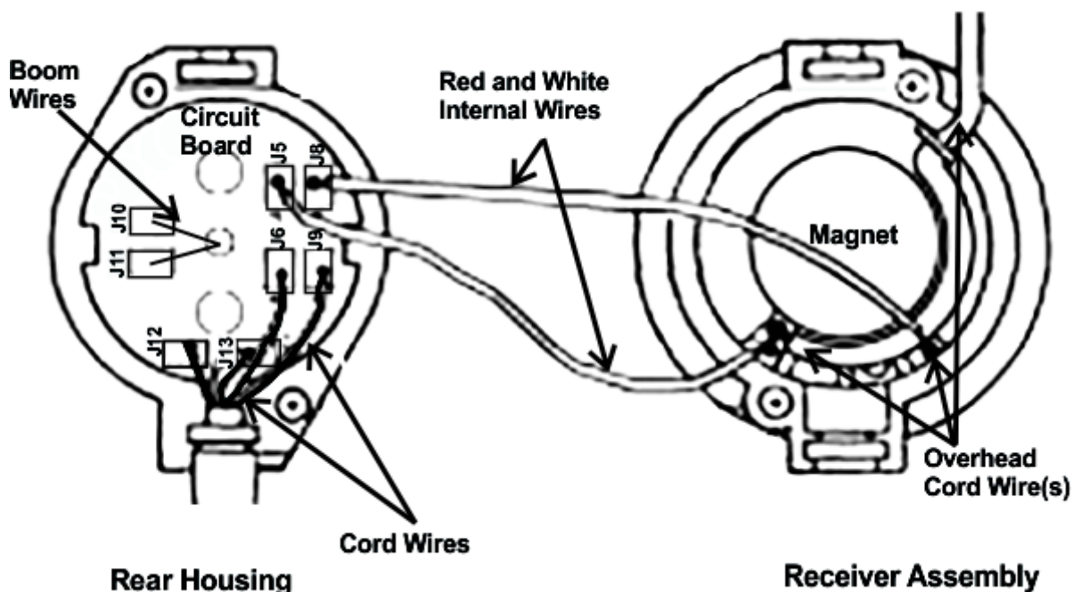
FIGURE 2. Circuit Board/Receiver/Cord Wiring
