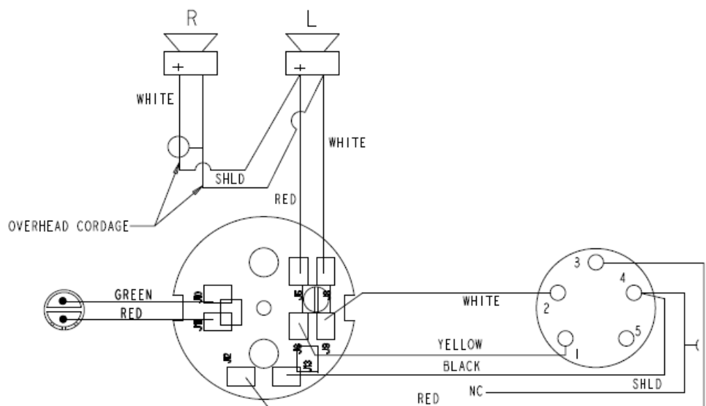
FIGURE 3. Airman 750 Headset Models -205, -208 Wiring Diagram
