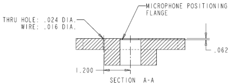
FIGURE 5. Flat Plate Coupler
