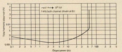
Output power vs. total harmonic distortion
