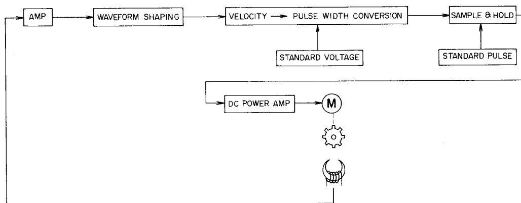
Fig. 5 Block Diagram
