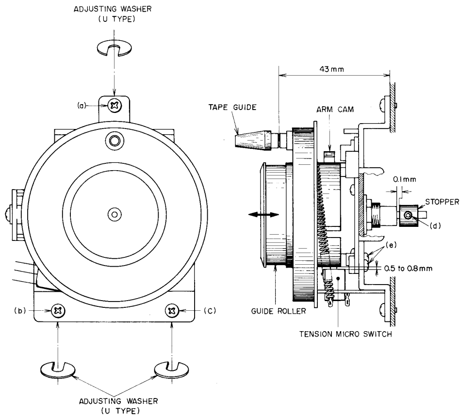
Fig. 8 Roller Block
