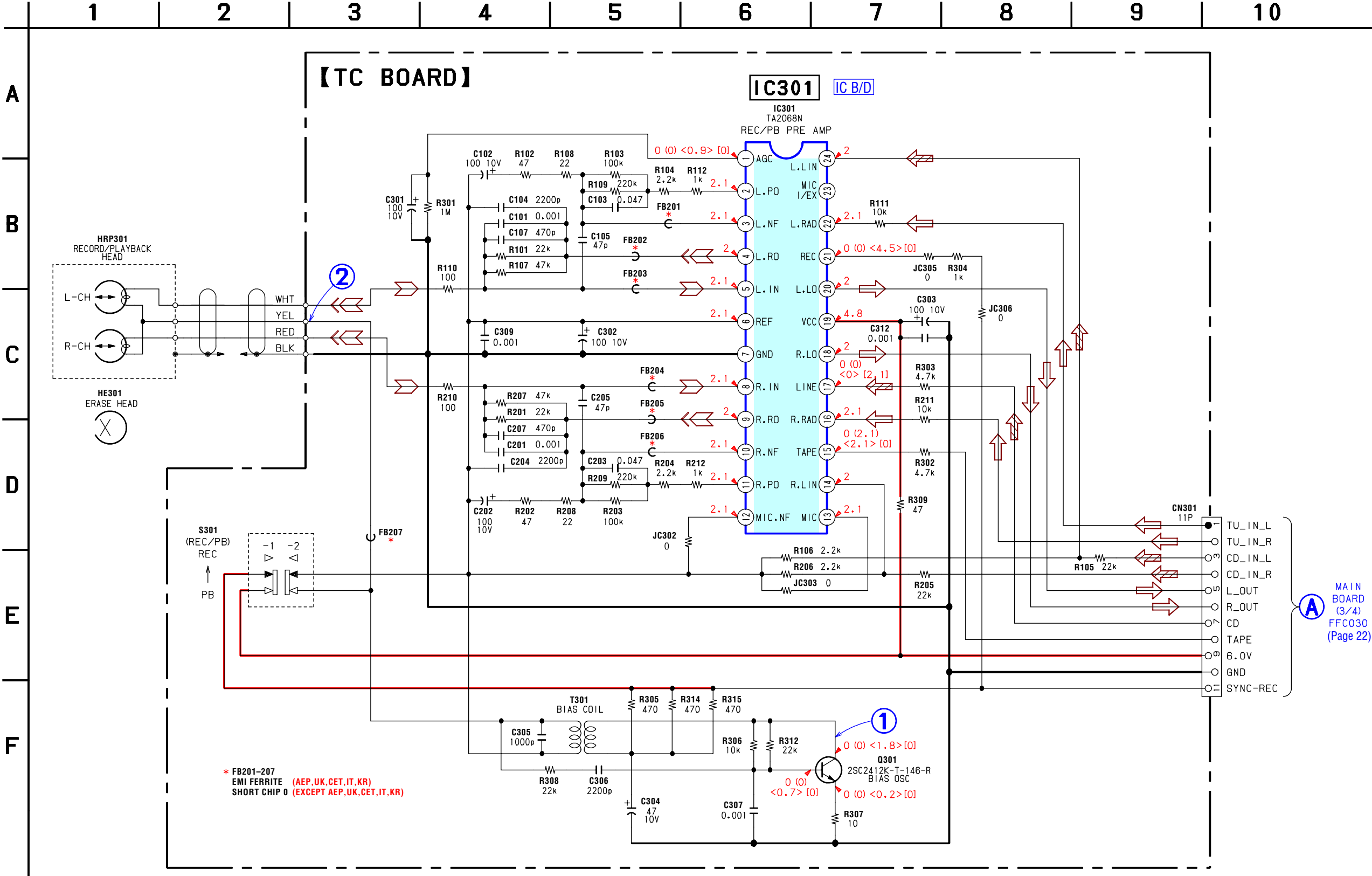
6-10. SCHEMATIC DIAGRAM — TC SECTION — • Refer to page 19 for Waveforms. • Refer to page 33 for IC Block Diagram.
