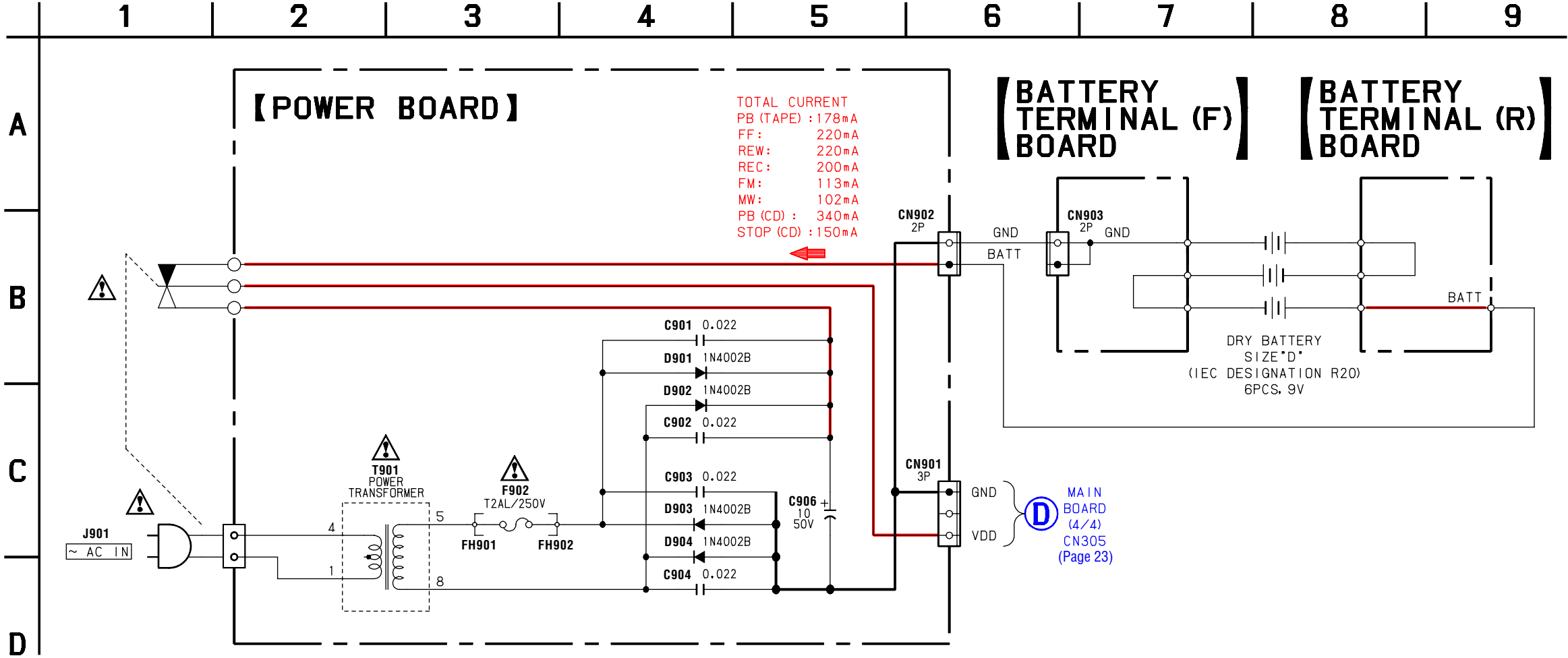
6-14. SCHEMATIC DIAGRAM — POWER SUPPLY SECTION —
