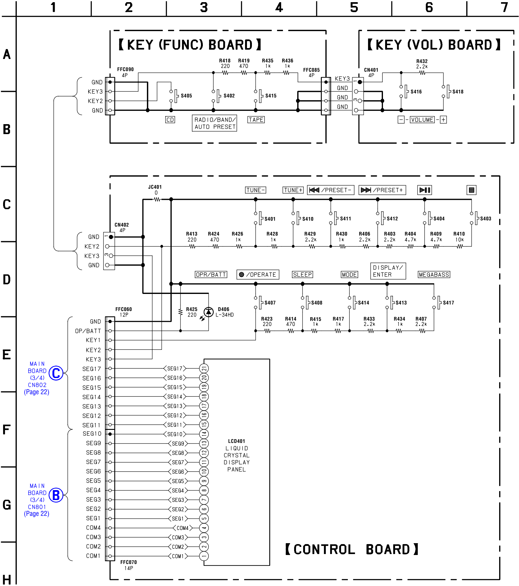
6-12. SCHEMATIC DIAGRAM — CONTROL SECTION —
