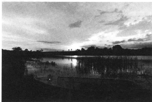
Centre-Weighted Metering
