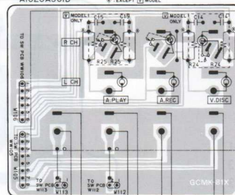
PIN JACK PCB A1020A501D
